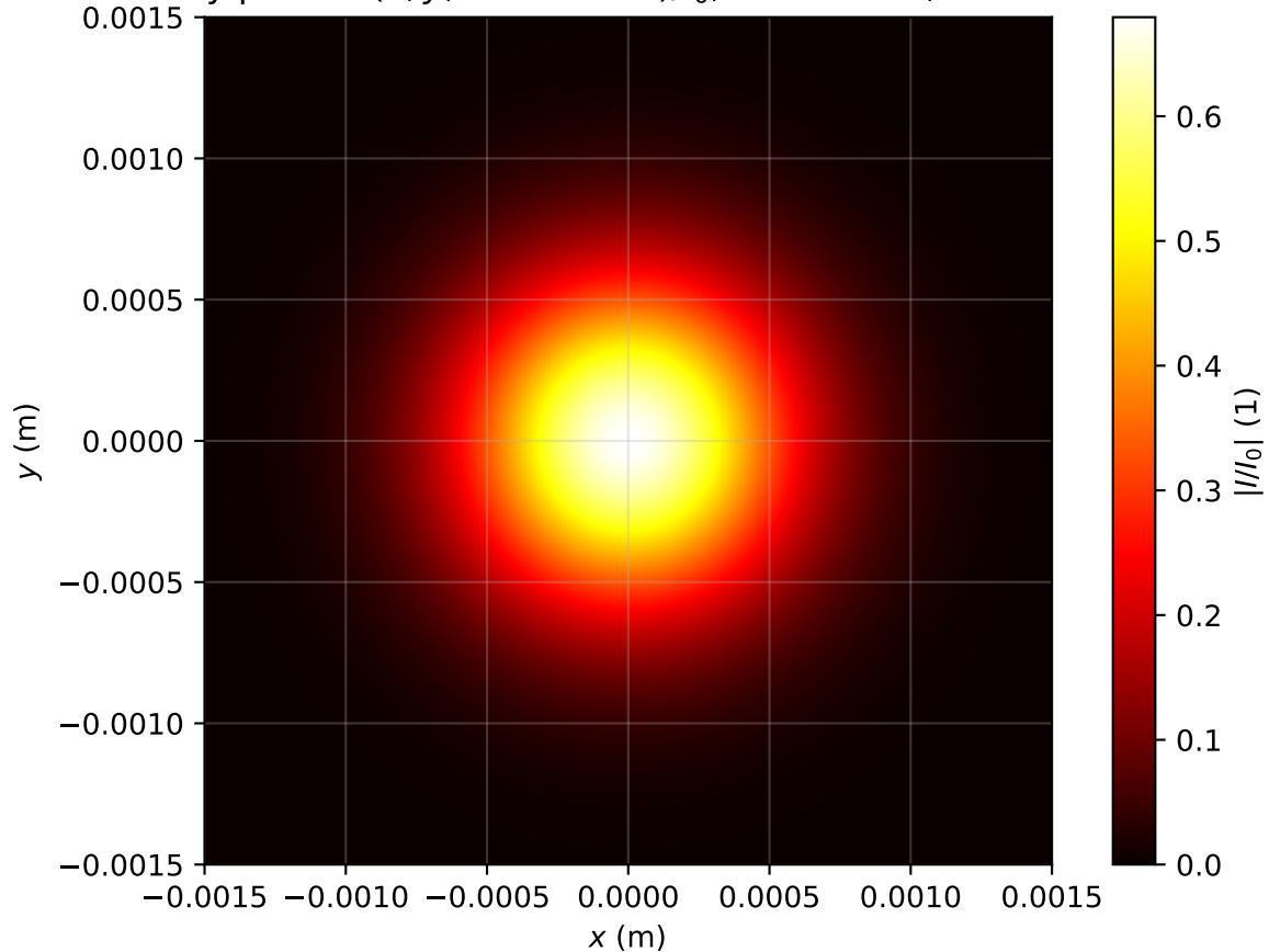
Intensity profile I(x, y, z = 1.513m)/I_0 , Pin=0.1Pcr, artificial time
